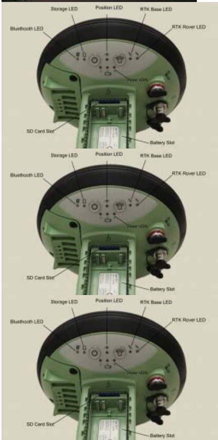
Setting up a pre-configured GS15 as an RTK base without the data logger
